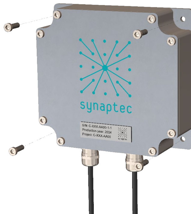
Figure 3.1: Arrangement of mounting holes on the PSC-1 base.
