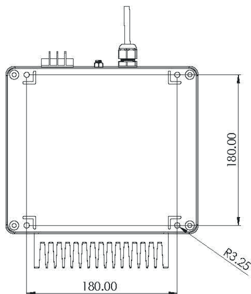
Figure 3.1: Arrangement of mounting holes on the S-PCT base.
