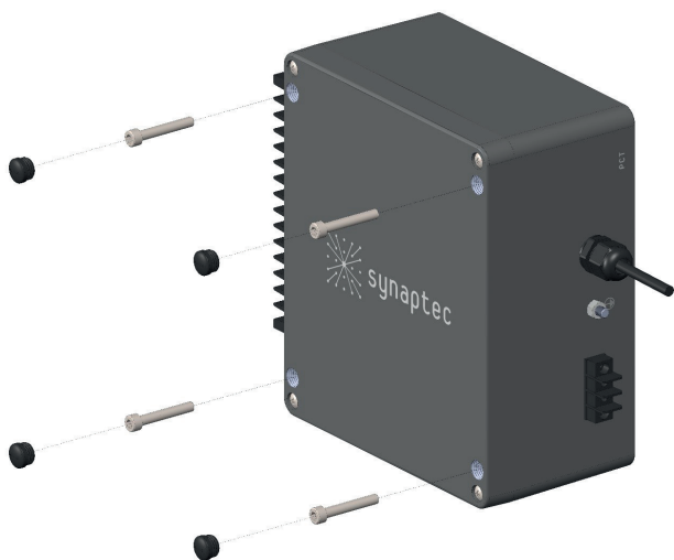
Figure 3.2: S-PCT mounting arrangement.
