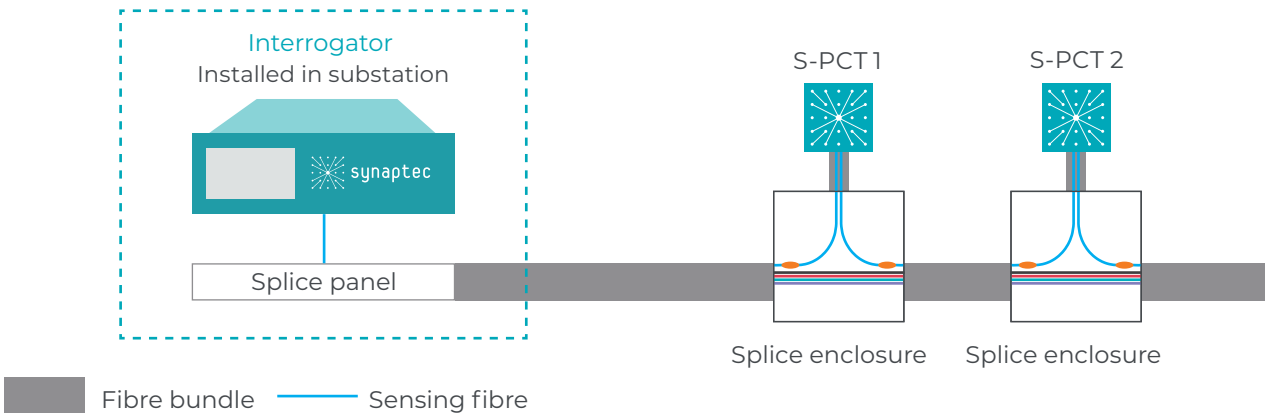
Figure 2.2: Example fibre routing between S-PCT units and central DES Interrogator.
