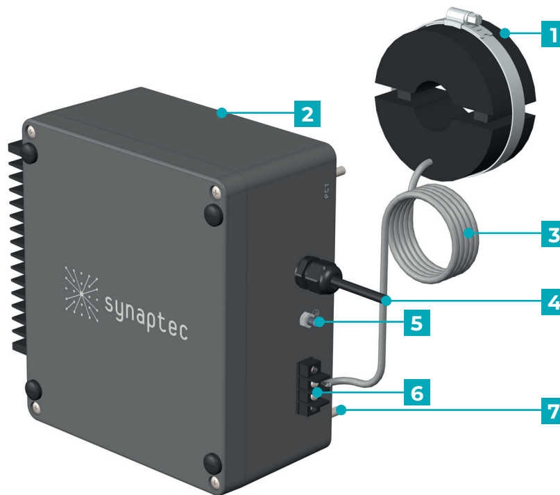
Figure 2.1: S-PCT design. Numbered items are identified in Table 2.1.
