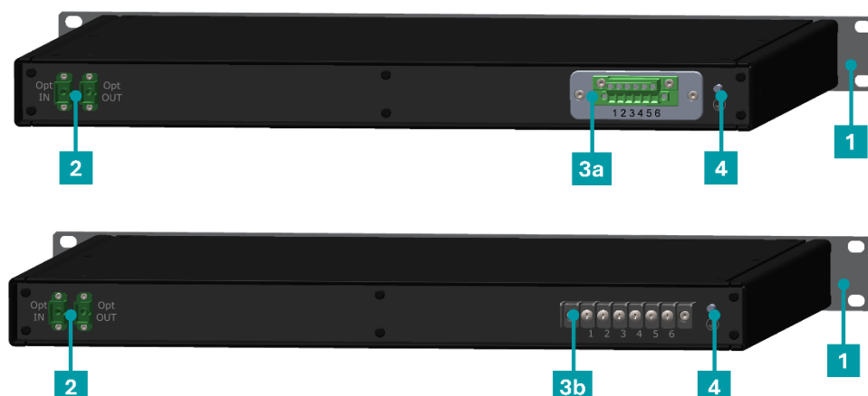
Figure 2.1: PSC-3 design. Numbered items are identified in Table 2.1. Please note both rear panel variants.
